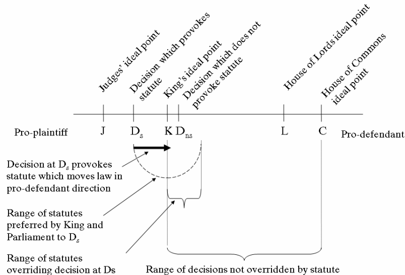
FIGURE 5 A SPATIAL MODEL OF LEGISLATIVE-JUDICIAL INTERACTION
